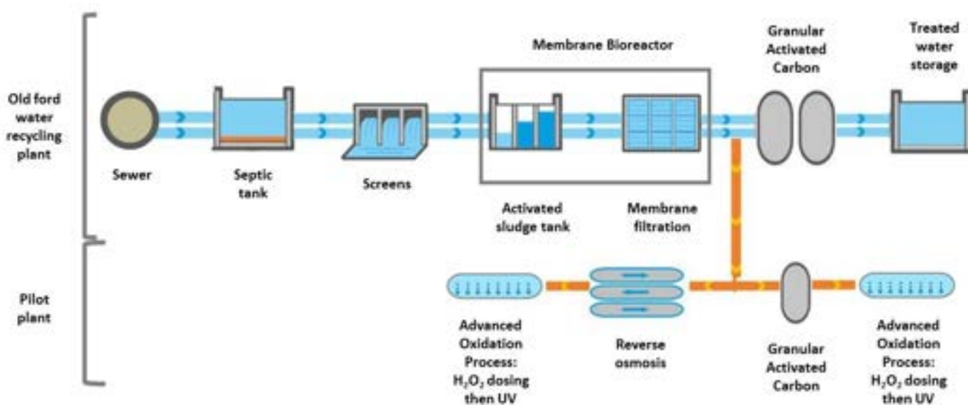
Figure 2: OFWRP and IPR pilot plant advanced treatment processes.
