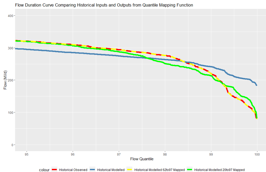
Figure I - 11: Flow Duration Curves for the historical observed (red) and historical modelled (blue) record, along with the mapped modelled historical (overlapping reference period, yellow dotted) and mapped modelled historical (non-overlapping reference period, green
