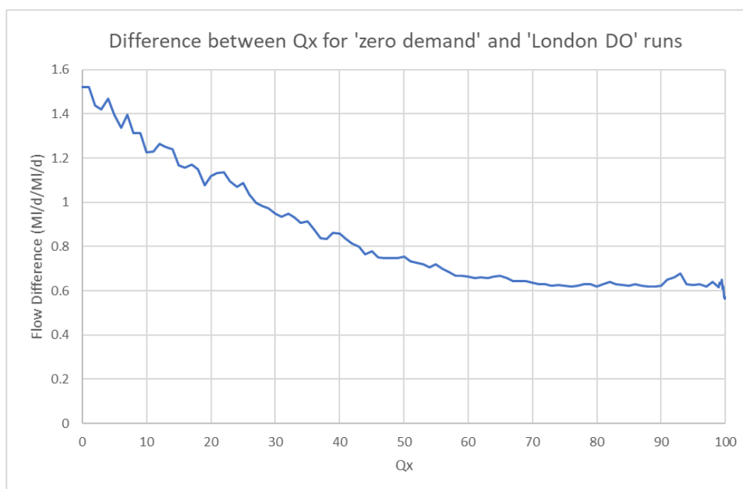
Figure I - 4: Example FDC-based Denaturalisation Curve
