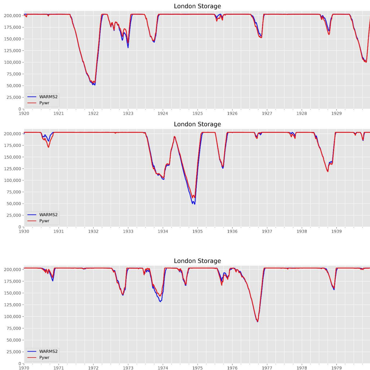
Figure I - 6: Step 1 Pywr Model Validation Plots
