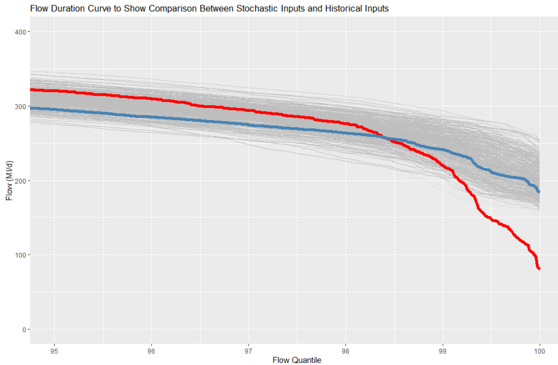
Figure I - 12: Flow Duration Curves for the historical observed (red), historical modelled (blue), and stochastic modelled (grey – 400 stochastic replicates)
