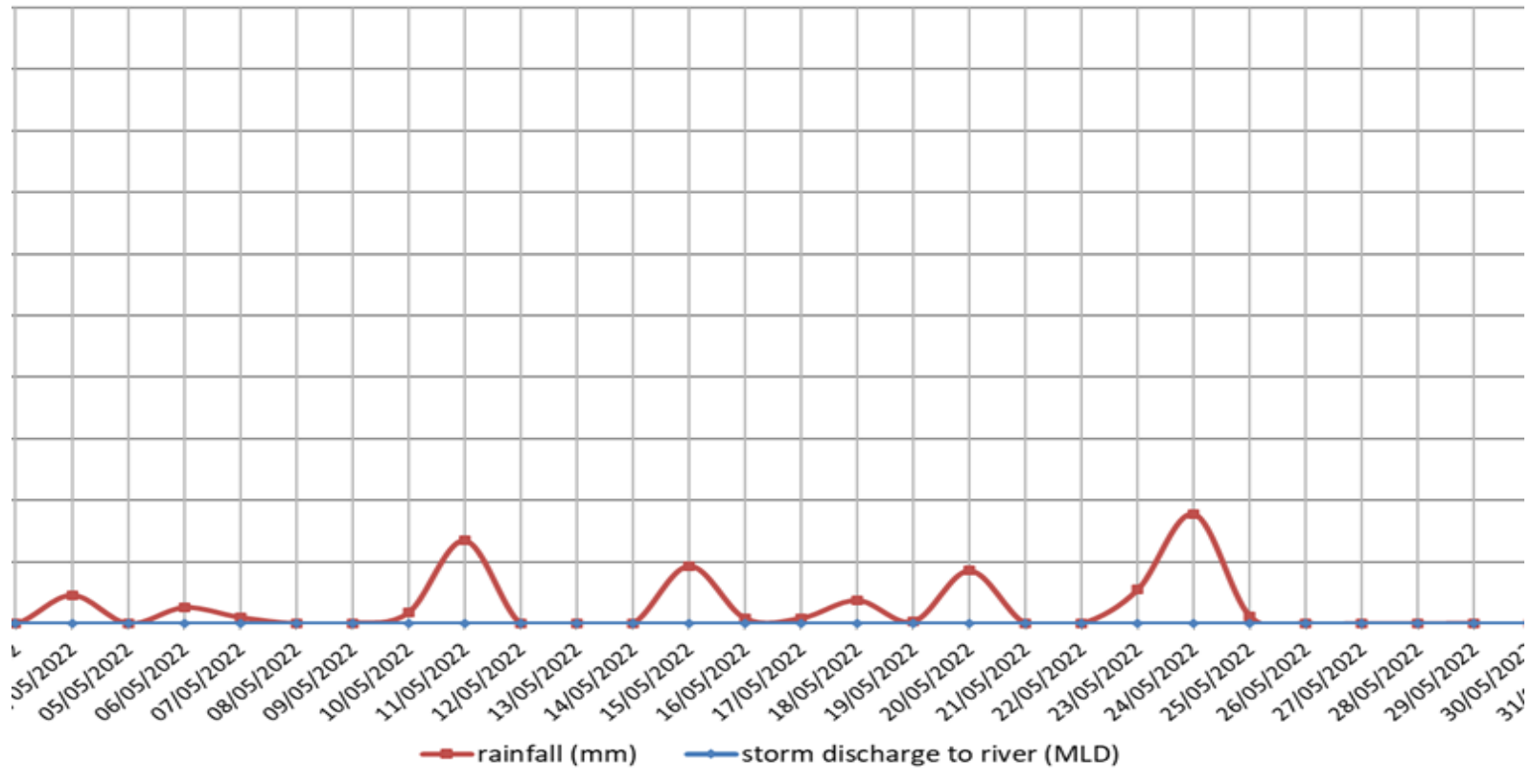
Mogden STW - Rainfall and Storm Flow to River (May 2022)
