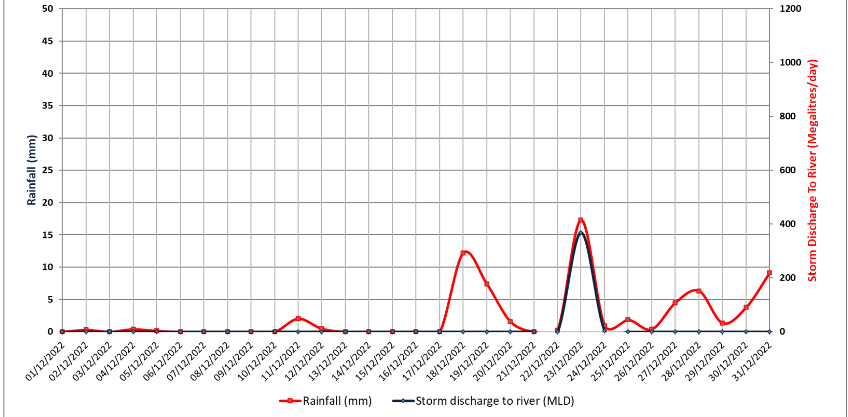
Mogden STW - Rainfall and Storm Flow to River (December 2022)
