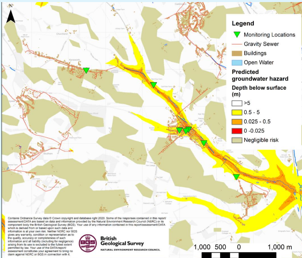
Figure 2.0 – Markyate monitoring area and infiltration zones
