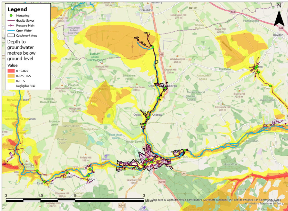
Figure 1 – Marlborough Monitoring Plan
