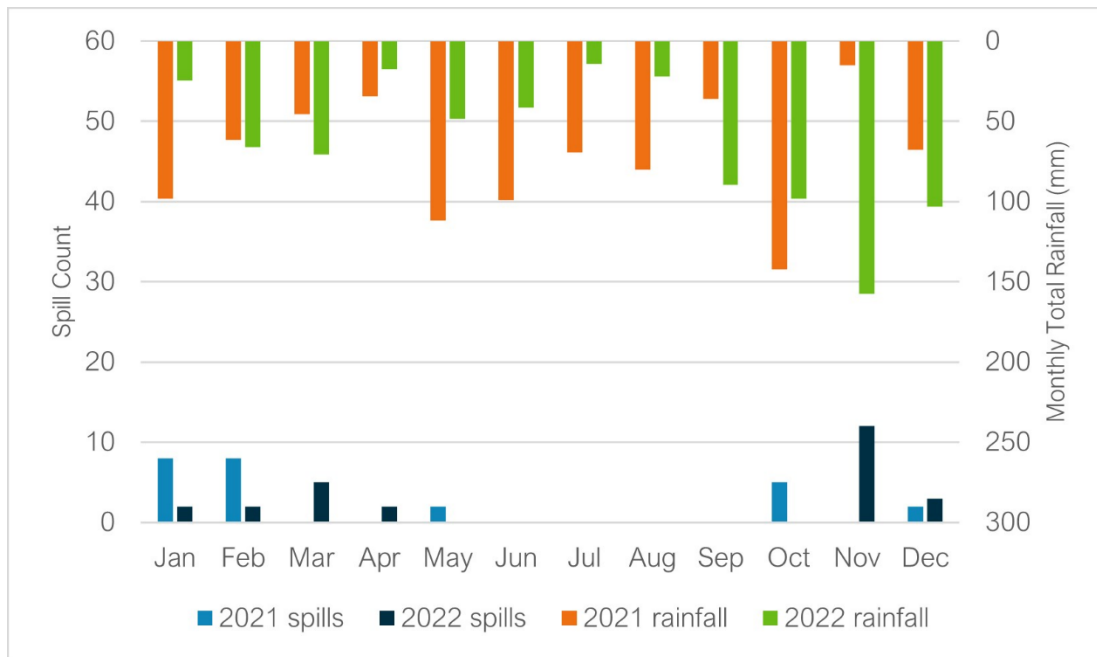
Figure 12 – EDM Monthly Performance – Knights Lane SPS
