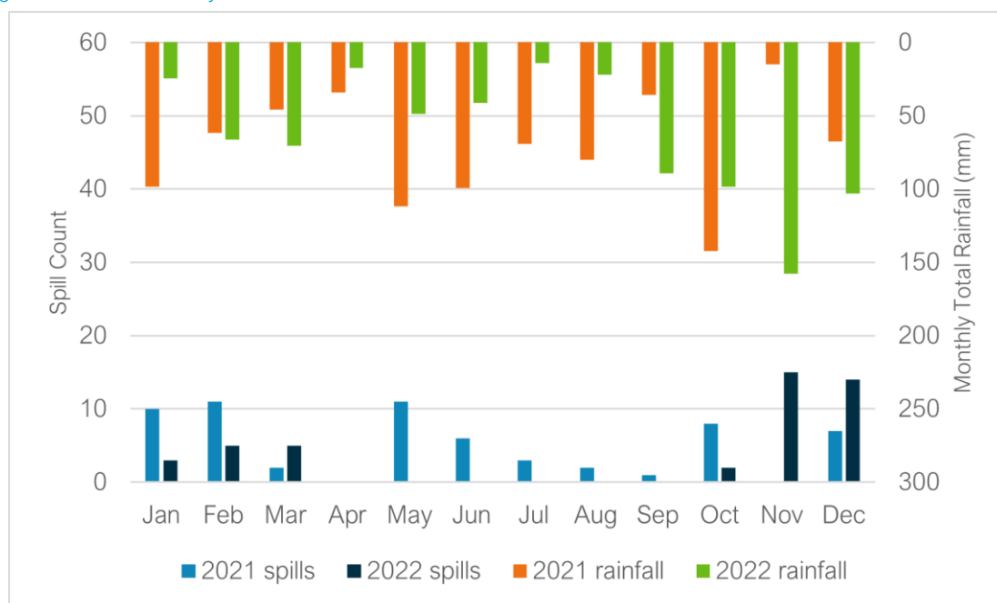
Figure 8 – EDM Monthly Performance – Wash Water STW
