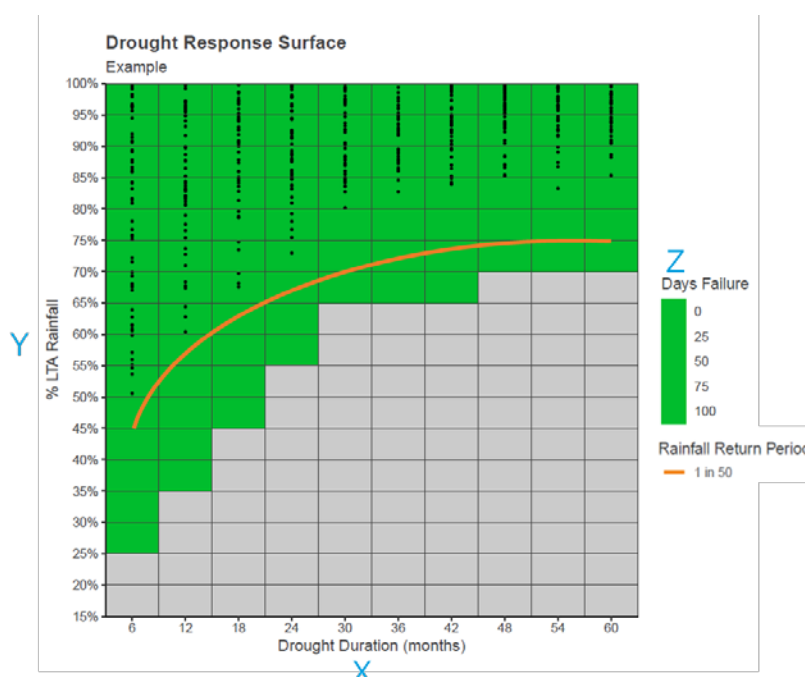
Figure 4 - 20: Example Drought Response Surface
