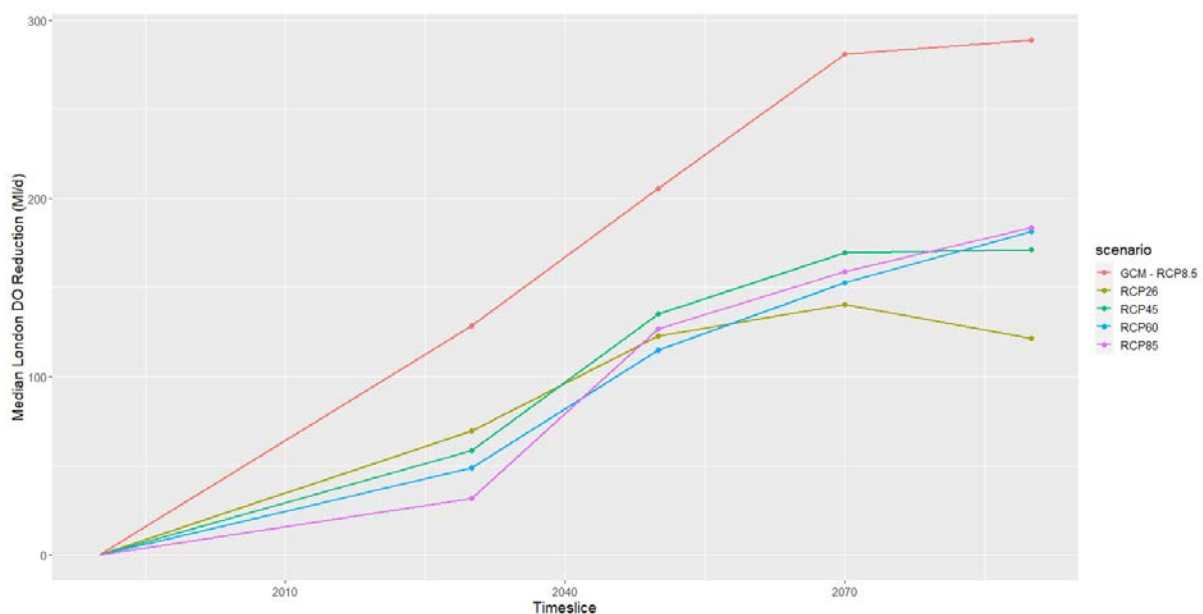
Figure 4 - 8: Median 1:500 DO Impacts from Each Combination of Timeslice and Emissions Scenario
