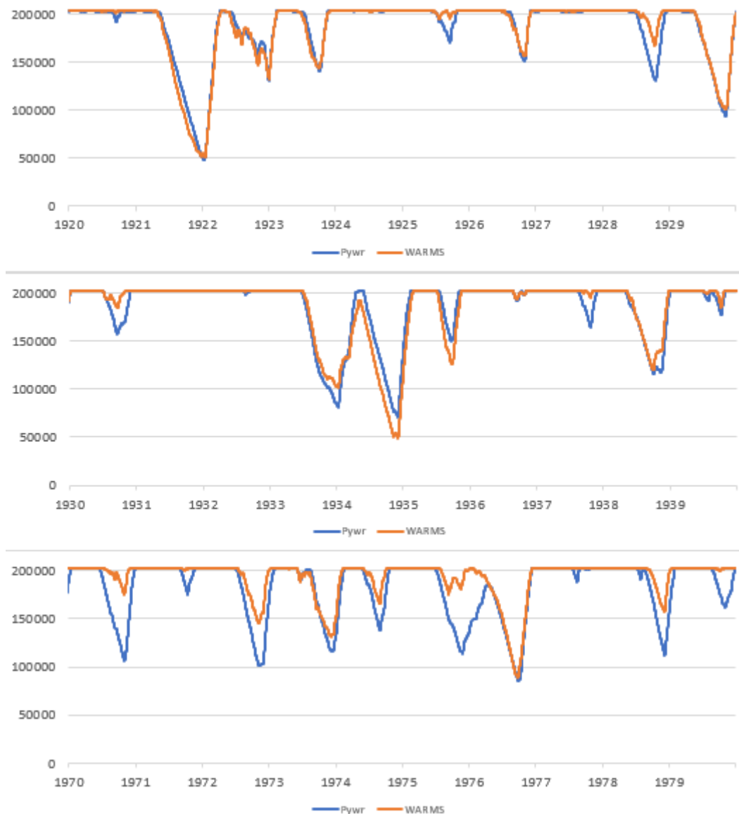
Figure I-7: Step 2 Pywr Model Validation Plots (y-axis is storage in MI)
