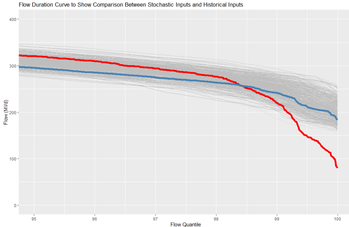
Figure I-12: Flow Duration Curves for the historical observed (red), historical modelled (blue), and stochastic modelled (grey – 400 stochastic replicates)
