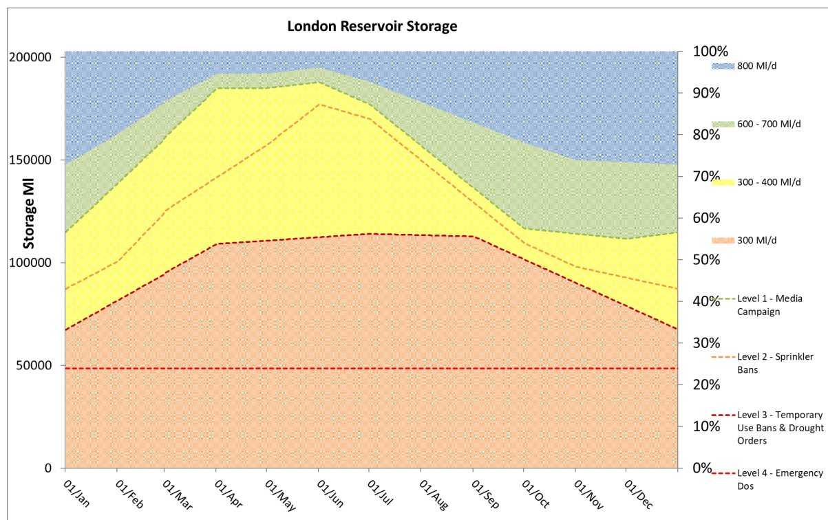
Figure I-1: Lower Thames Control Diagram
