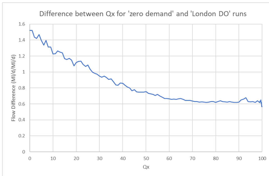
Figure I-4: Example FDC-based Denaturalisation Curve
