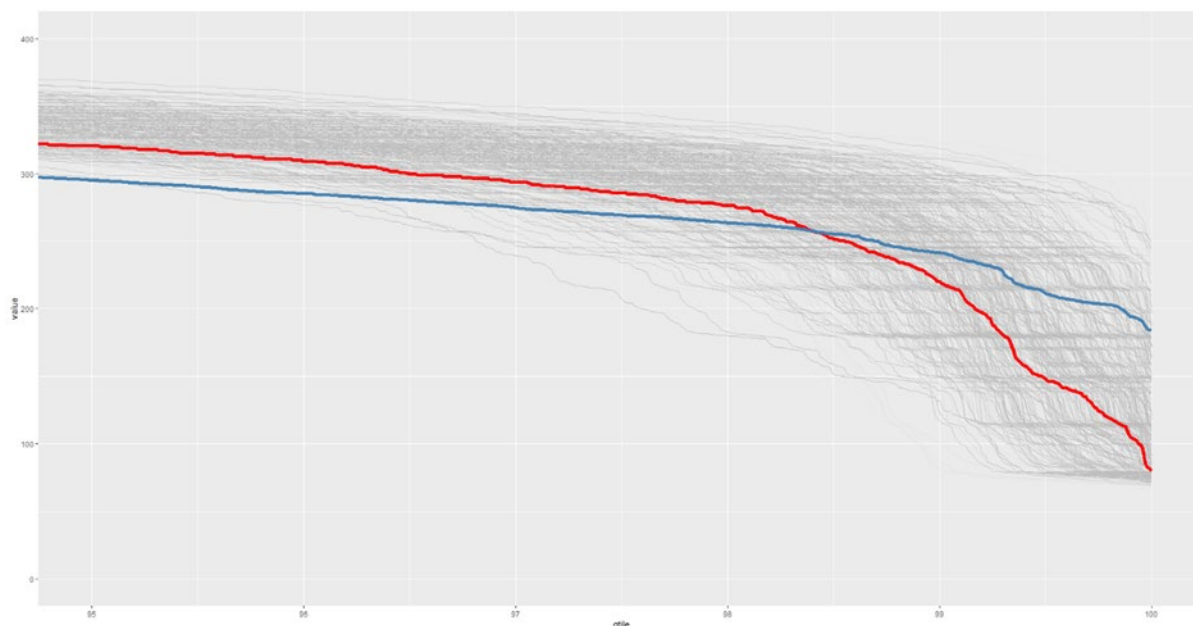
Figure I-13: Flow Duration Curves for the historical observed (red), historical modelled (blue), and mapped stochastic modelled (grey – 400 stochastic replicates) – low flow focus
