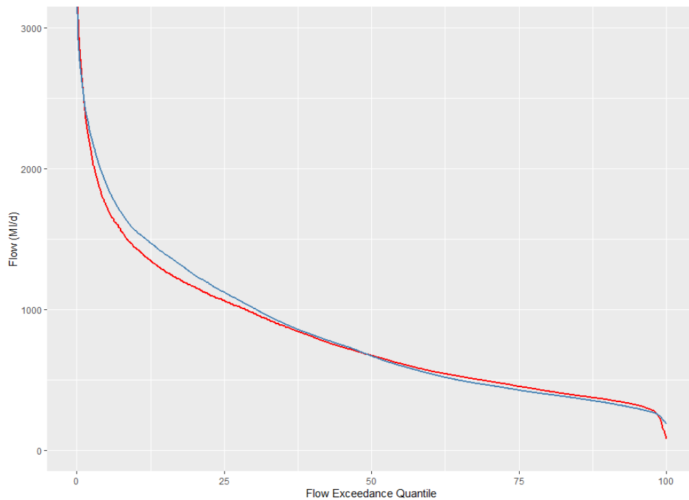
Figure I-8: Flow-Duration Curves for the Historical Observed (red) and Modelled (Blue) Record
