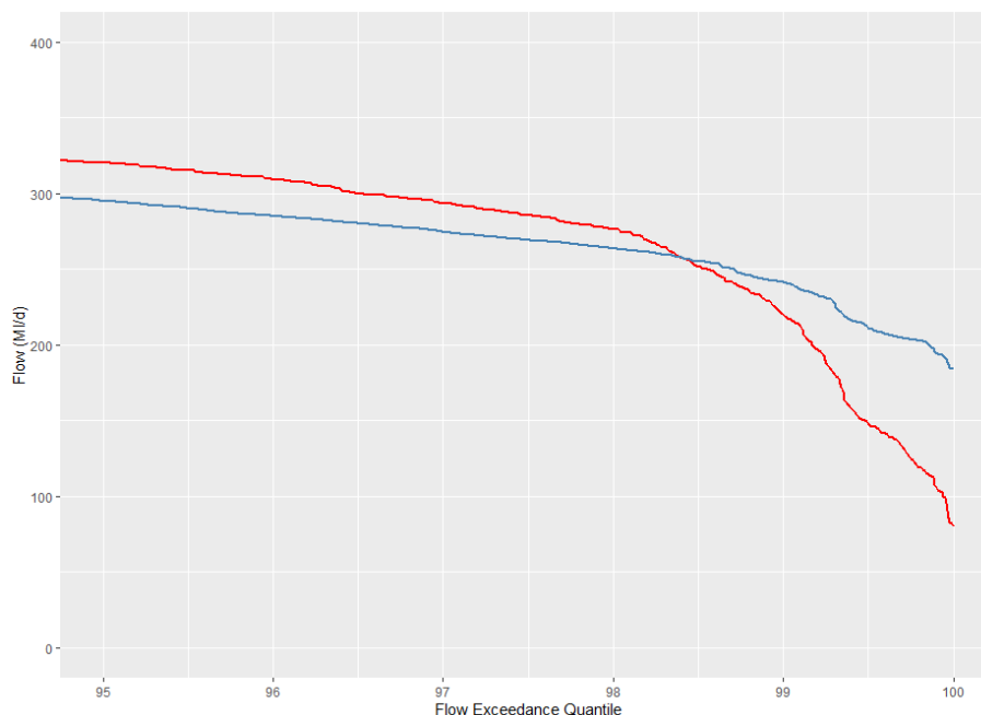
Figure I-10: Flow Duration Curves for the historical observed (red) and modelled (blue) record – low flow focus
