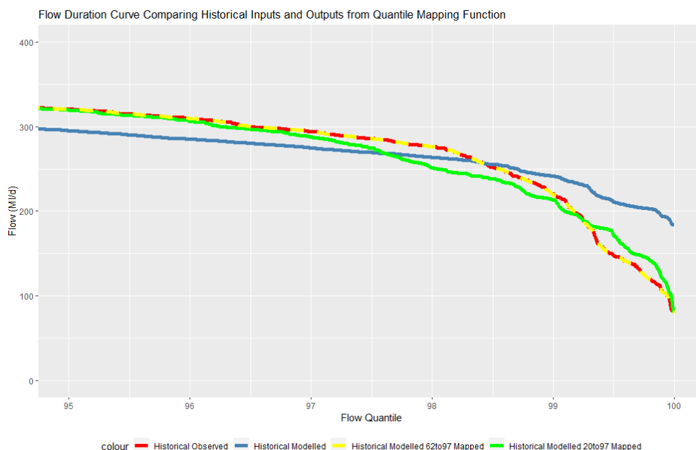
Figure I-11: Flow Duration Curves for the historical observed (red) and historical modelled (blue) record, along with the mapped modelled historical (overlapping reference period, yellow dotted) and mapped modelled historical (non-overlapping reference period, green)
