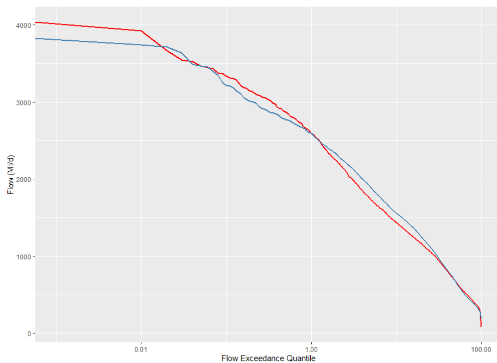
Figure I-9: Flow Duration Curves for the historical observed (red) and modelled (blue) record
