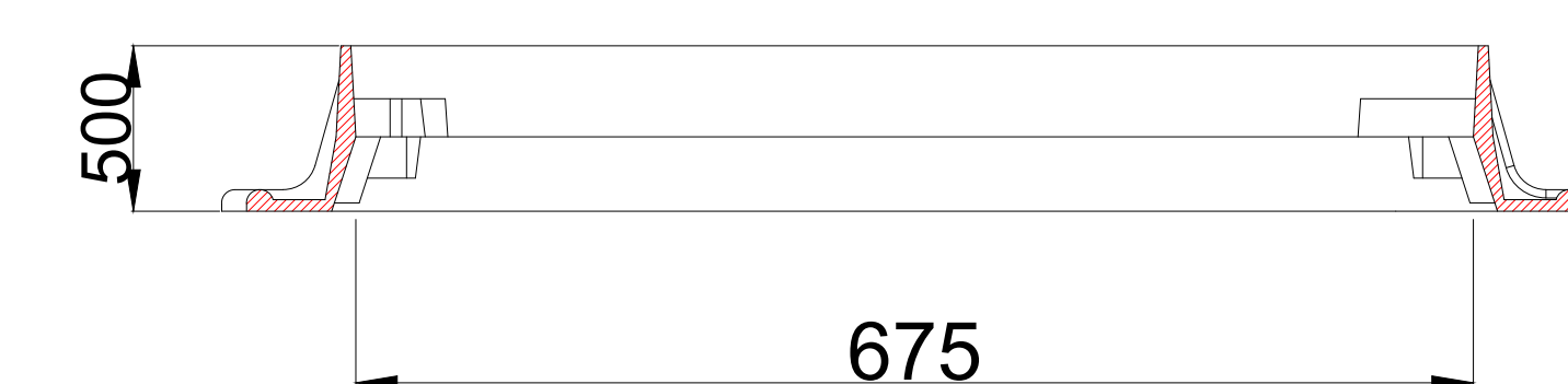
SECTION C-C
