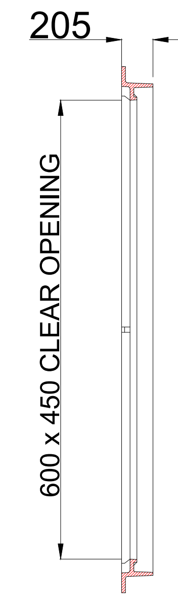
SECTION C-
