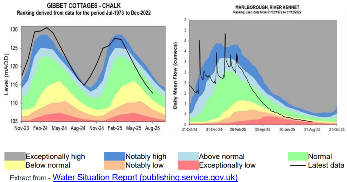
Figure 6 – Ground Water Situation Report
