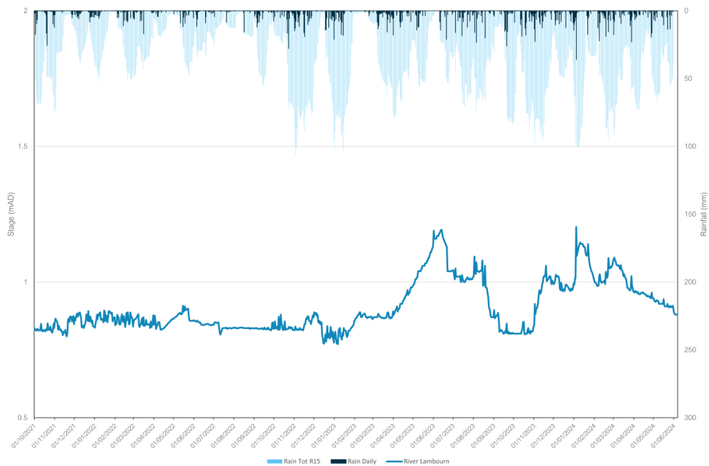
Figure 5A – River Lambourn at Lambourn
