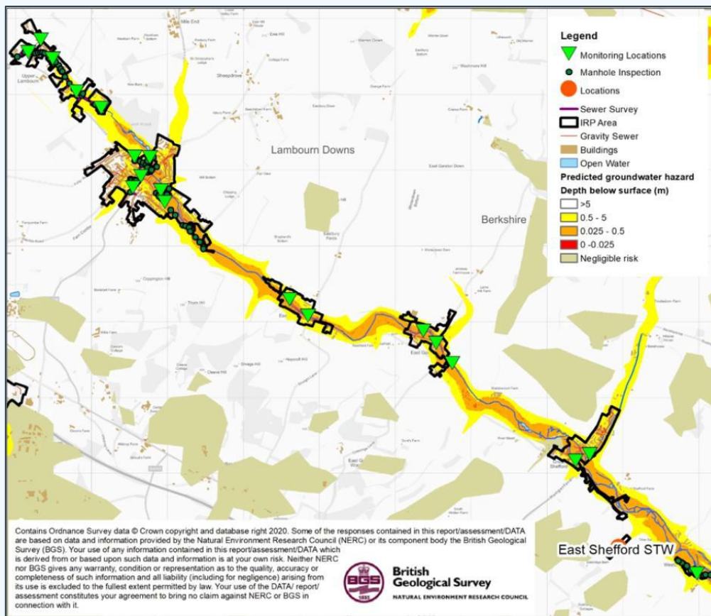
Figure 1: Ramsbury monitoring and infiltration zones
