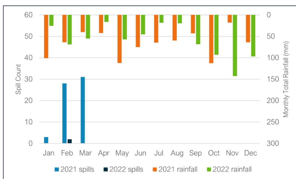
Figure 10 – EDM Monthly Performance
