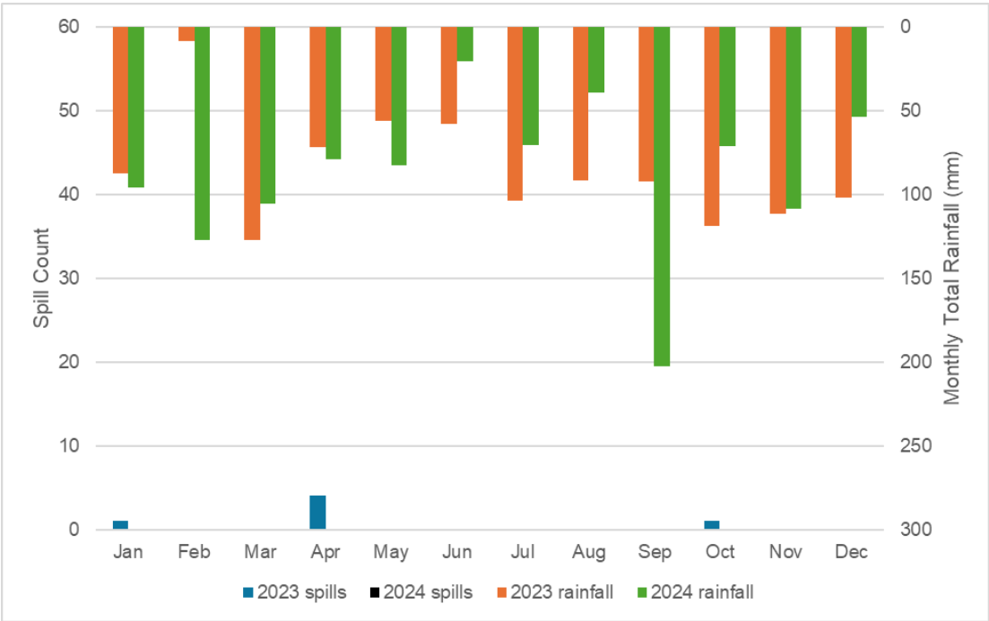
Figure 10 – Monthly rainfall data versus monthly spill count for 2023 and 2024 at East Garston STW
