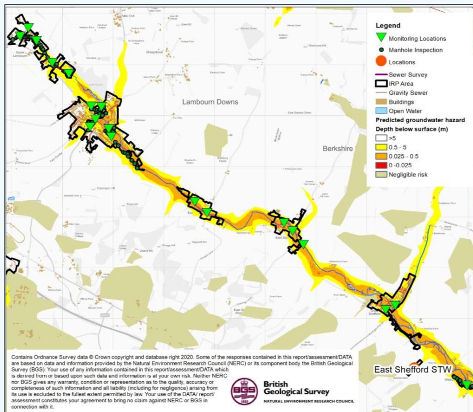
Figure 2.0 – East Shefford monitoring and infiltration zones
