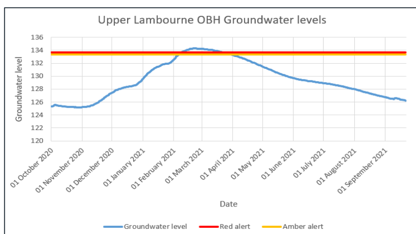
Figure 4 – 2020/21 Groundwater Levels at Upper Lambourn Observation Borehole (OBH)
