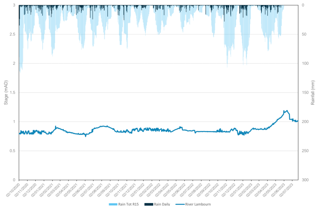
Figure 5A – River Lambourn at Lambourn
