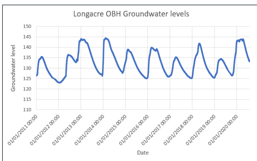
Figure 5 – 2011-2021 Groundwater Levels at Longacre Observation Borehole (OBH) (more complete data for this time period than Upper Lambourn OBH).
