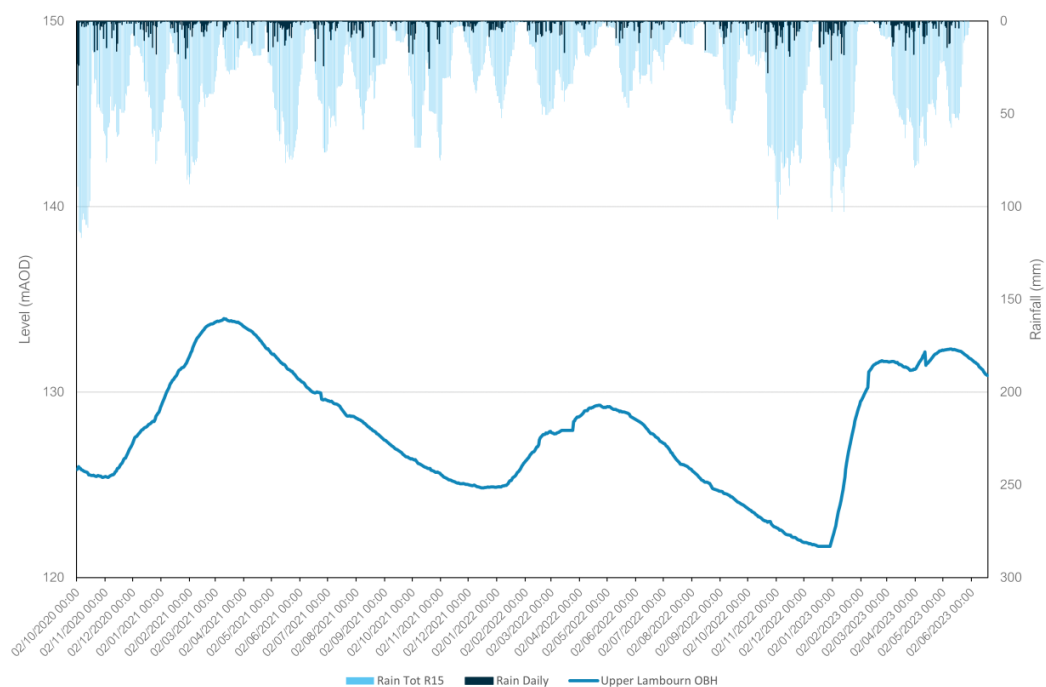
Figure 5B – Upper Lambourn OBH
