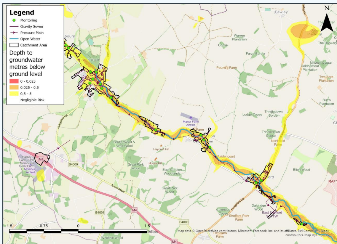
Figure 1: East Shefford Monitoring Plan
