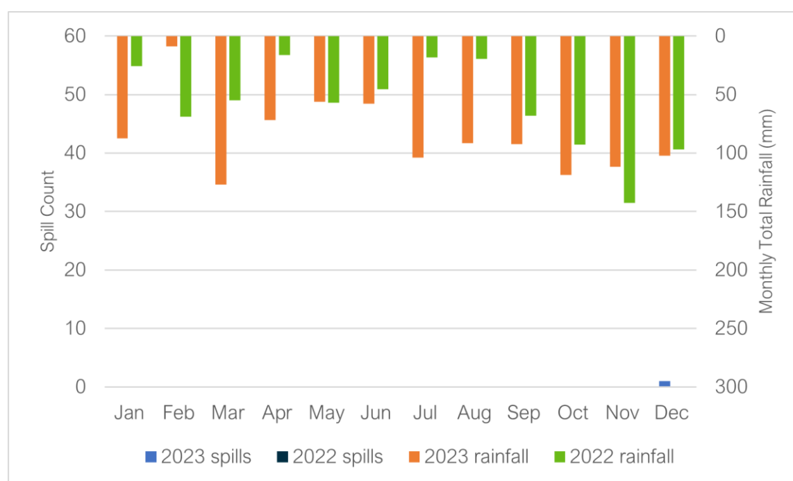
Figure 10 – EDM Monthly Performance at East Garston STW
