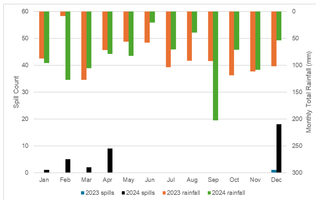
Figure 8 – Monthly rainfall data versus monthly spill count for 2023 and 2024 at East Shefford STW
