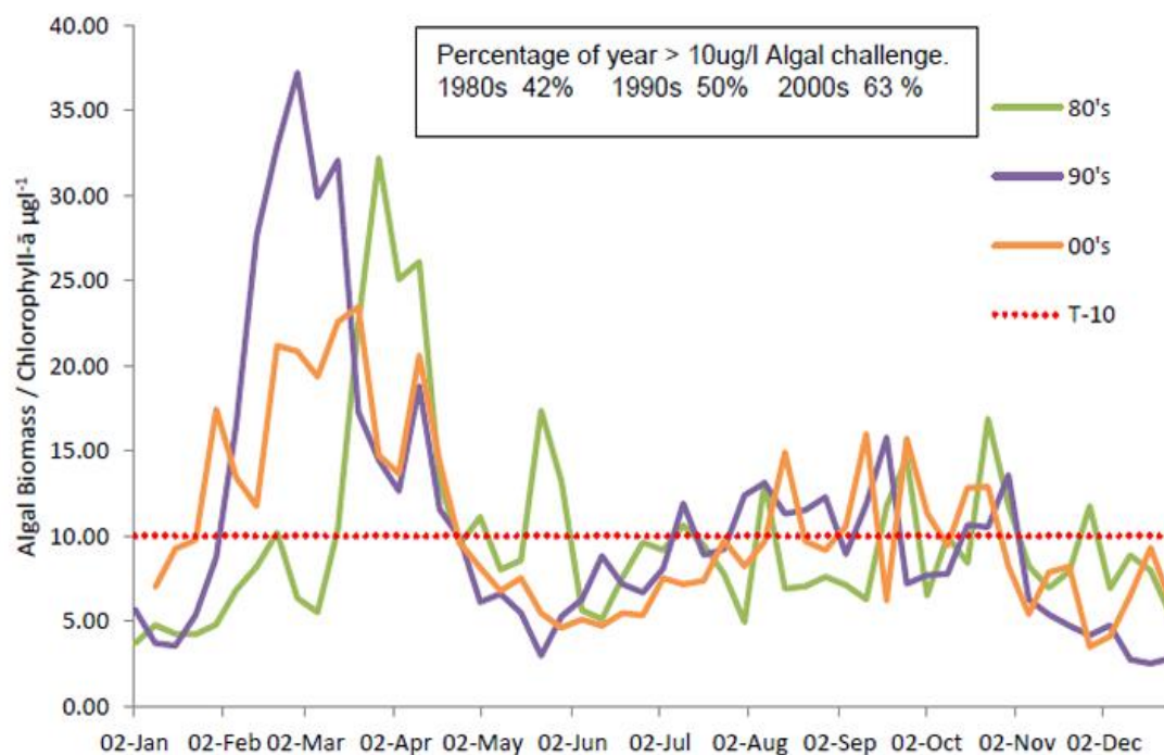
Figure K - 1: Decadal pattern of changing algal blooms 5
