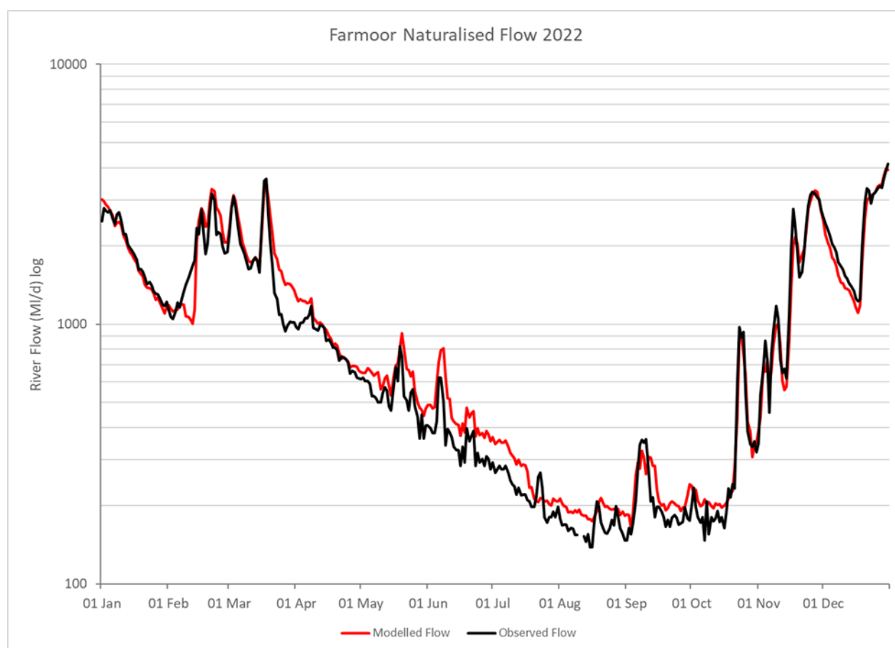
Figure CC-3: Modelled and Observed Farmoor Flows from the 2022 Drought
