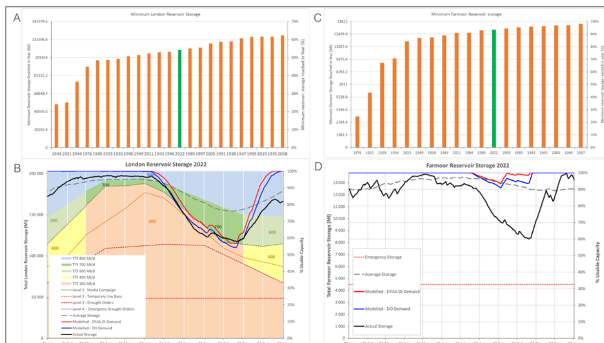
Figure CC-2: A. Minimum modelled London storage reached in different drought events. B. Observed and modelled London reservoir storage in 2022. C. Minimum Farmoor Storage Reached in Different Drought Events. D. Observed and modelled Farmoor storage in 2022
