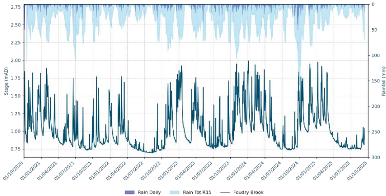
Figure 3: River Level data for Foudry Brook, Beech Hill
